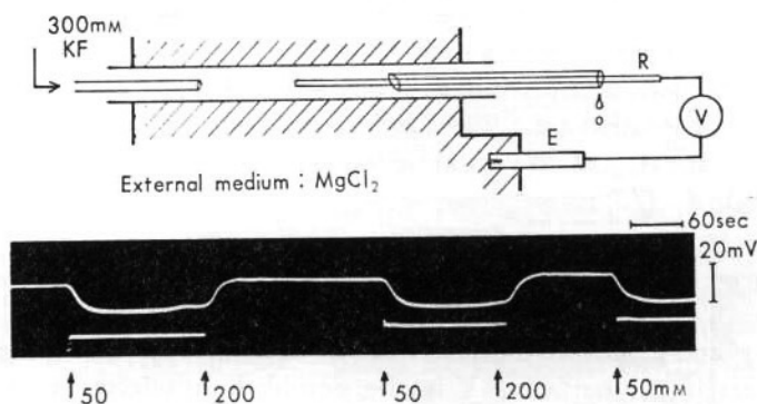
Fig. 2. Top : Schematic diagram showing the experimental setup used to determine the effect of the external divalent cation concentration on the resting membrane potential; E represents a calomel electrode and R a glass capillary electrode filled with 600 mM KCl. Bottom : Oscillograph records taken from an axon internally perfused with 300 mM KF (glycerol) solution (phosphate buffer). Downward deflections represent increased negativity within the axon. External media are prepared by mixing a 400 mM MgCl_2 (Tris-buffer) with 12% (v/v) glycerol (Tasaki, Watanabe and Lerman, Am. J. Physiol. , 213 , 1465 (1967)).
