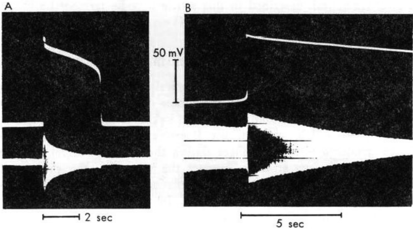
Fig. 7. A: Changes in the membrane impedance associated with the electrically induced action potential of an axon internally perfused with 25 mM CsF solution and immersed in 200 mM \text{CaCl}_2 solution. The impedance bridge was balanced with the membrane impedance in the resting state. The room temperature was 18°C. B: Changes in the membrane impedance produced by an alteration of the composition of the external medium from a mixture of 200 mM \text{CaCl}_2 and 25 mM CsCl to a mixture of 100 mM \text{CaCl}_2 and 450 mM CsCl (abrupt depolarization). The temperature was 19°C. Note that the sudden rises in the membrane potential were associated with simultaneous changes in the membrane impedance (Tasaki, Takenaka and Yamagishi, Am. J. Physiol. , 215 , 152 (1968)).
