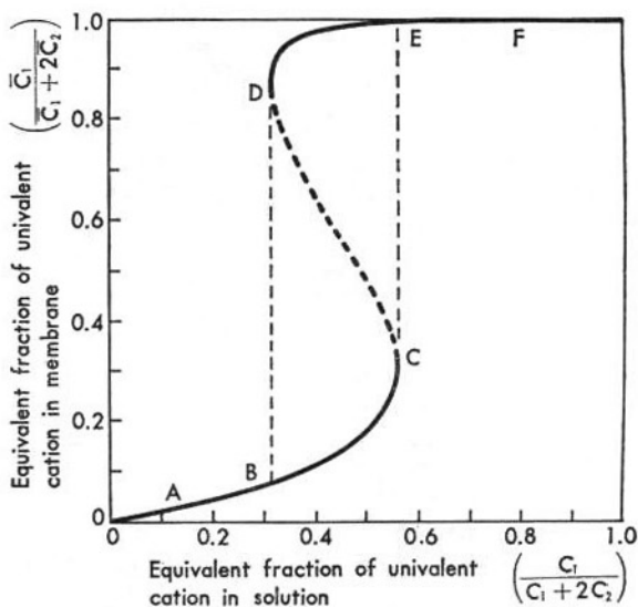
Fig. 6. Theoretical ion exchange isotherm calculated for a cation exchanger membrane immersed in a salt solution containing univalent and divalent cations. In the calculation, it was assumed that occupancy of two neighboring charged sites in the membrane by two cations of different valences is energetically unfavorable. C_1 and C_2 represent the concentrations in the solution of univalent and divalent cations, respectively; \bar{C}_1 and \bar{C}_2 represent the concentrations within the membrane. When the equivalent fraction of the univalent cation in the solution is increased continuously from 0 to 1, the corresponding fraction in the membrane increases along the course 0, A, B, C, E, and F. When the equivalent fraction in the solution is decreased from 1 to 0, the corresponding fraction in the membrane changes along F, E, D, B, A, and 0 (Lerman, Watanabe and Tasaki, in "Neurosciences Research," ed. by Ehrenpreis and Solnitzky, Academic Press, New York, Vol. 2, p. 71 (1969)).
