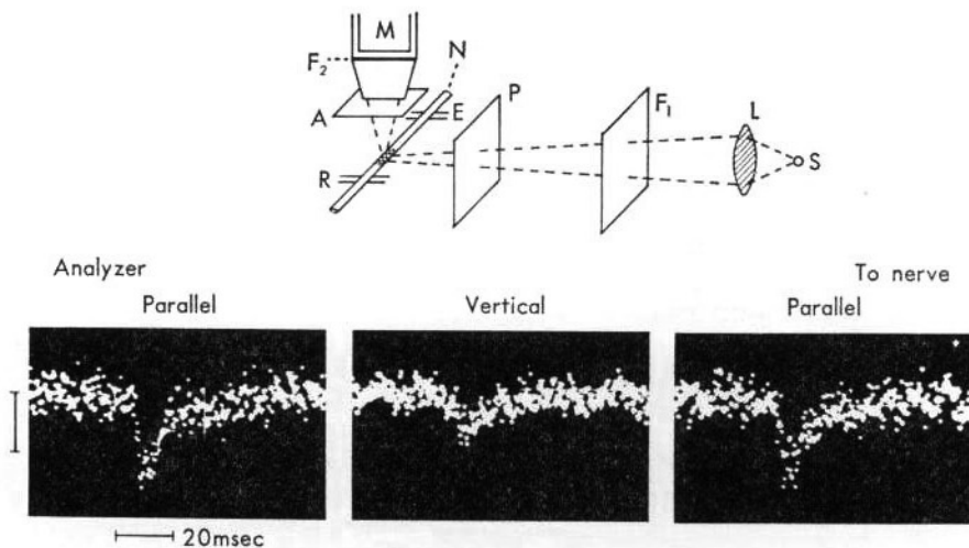
Fig. 8. Top ; Schematic diagram showing the experimental setup used to measure changes in fluorescence polarization during excitation in a crab nerve stained with Pyronin B. The letter S represents the light source; L, lens; F_1 , primary filter; F_2 , secondary filter; M, photomultiplier tube; P, polarizer; A, analyzer; N, nerve; E, stimulating electrodes; R, recording electrodes. Bottom ; Optical signals obtained with the principal axis of the analyzer (E-vector of fluorescent light) parallel to the long axis of the nerve (right and left records) and perpendicular to the nerve (middle record). The quasi-monochromatic light used for excitation of dye molecules was polarized with its E-vector in the direction parallel to the nerve. A CAT computer was used for recording. For right and left records, the vertical bar represents 2 \times 10^{-4} times the background intensity. The middle record was taken under the same experimental conditions except that the analyzer was rotated by 90^\circ . The temperature was 19^\circ\text{C} (adopted from Tasaki, Carnay and Watanabe, Proc. Natl. Acad. Sci. U. S. , 64 , 1362 (1969)).
